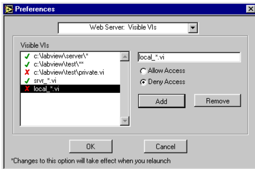
Figure 2-7. Web Server Visible VIs Dialog Box
